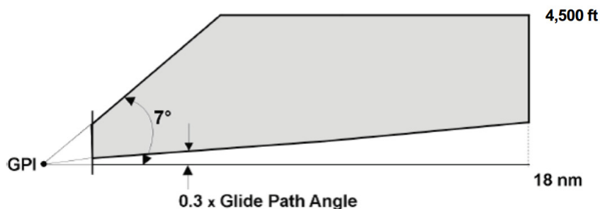
TLS LOCALIZER COVERAGE IN ELEVATION
